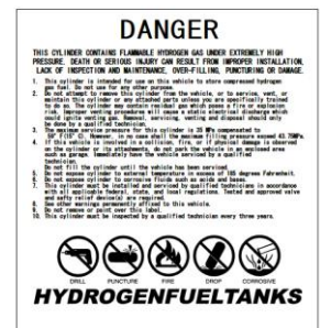
Label on outside of hydrogen tank
