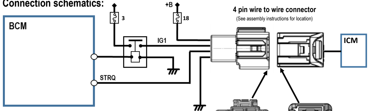
Fuse locations: Under dashboard fuse box
