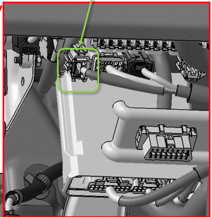
4 pin wire to wire connector
